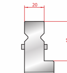
Wila New Standard Punch
